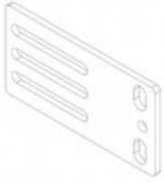
1 x Flat Vertical Bracket (250-70-0007-00) Dimensions (WxHxD): 85.2mm x 43.6mm x 3mm
