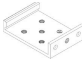
1 x Holder (250-80-0008-00) Dimensions (WxHxD): 61.46mm x 43.6mm x 16mm
