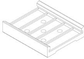
Sliding Bracket (250-70-0106-00)
