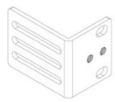
1 x L Bracket (250-70-0093-01) Dimensions (WxHxD): 38mm x 53mm x 43mm
