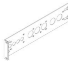
1 x L Bracket (250-70-3017-00) Dimensions (WxHxD): 365.23mm x 88.1mm x 21.3mm
