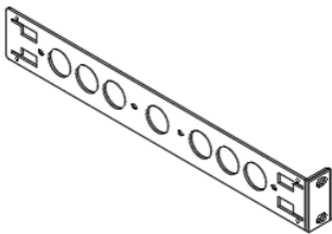
1 x L Bracket (250-80-0123-00) Dimensions (WxHxD): 305.48mm x 43.6mm x 21.3mm
