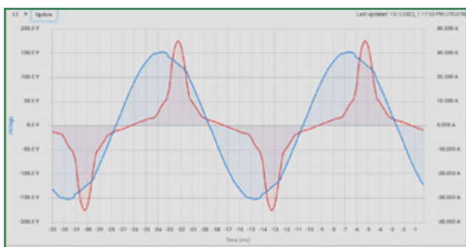
Harmonics Waveform Example
