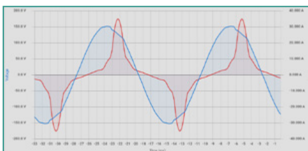
Harmonics Waveform Example
