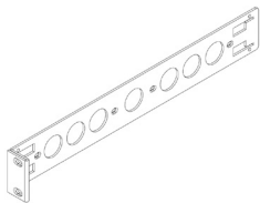
1 x L Bracket (250-80-0123-00) Dimensions (WxDxH): 305.48mm x 43.6mm x 21.3mm
