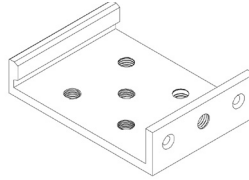
1 x Holder (250-80-0008-00) Dimensions (WxDxH): 61.46mm x 43.6mm x 16mm
