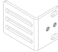
1 x L Bracket (250-70-0093-01) Dimensions (WxDxH): 38mm x 53mm x 43mm
