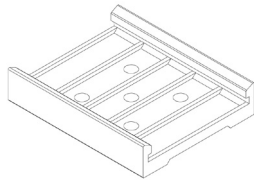
1 x Plastic Sliding Bracket (250-70-0106-00) Dimensions (WxDxH): 52mm x 13mm x 67mm
