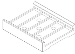
1 x Plastic Sliding Bracket (252-67-0029-00) Dimensions (WxDxH): 52mm x 13mm x 67mm
