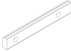
1 x Pin Bracket (250-80-0009-00) Dimensions (WxDxH): 43.6mm x 6.6mm x 3.2mm
