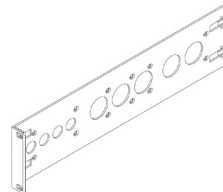
1 x L Bracket (250-70-3017-00) Dimensions (WxDxH): 365.23mm x 88.1mm x 21.3mm
