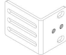
1 x L Bracket (250-70-0093-01) Dimensions (WxDxH): 38mm x 53mm x 43mm
