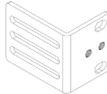
1 x L Bracket (250-70-0093-01) Dimensions (WxDxH): 38mm x 53mm x 43mm
